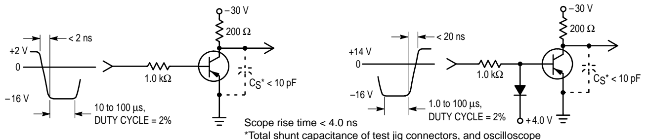
Figure 1. Turn–On Time
